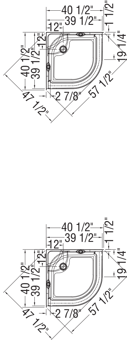
MAAX IES 1/2 positioning
